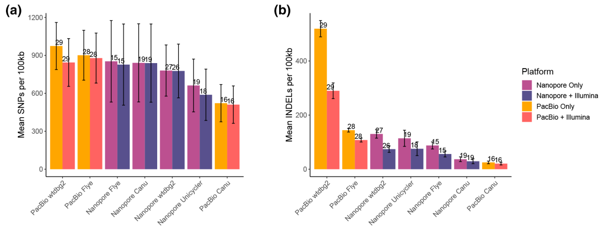
Fig. 5. Effect of polishing on error rate. SNPs and INDELs were identified in contigs from nanopore only, nanopore contigs polished with illumina reads, PacBio only and PacBio contigs polished with illumina reads. The number of SNPs (a) and INDELs (b) are expressed as the number per 100 kb of reference genome, where at least 50% of the reference genome was recovered by contigs, where at least 50% of the reference genome was recovered by contigs. Error bars are standard error of the mean, and the number above the bar indicates the number of genomes included in the mean calculation [from a total possible maximum of 60 (15 genomes, 4 assemblies)].
